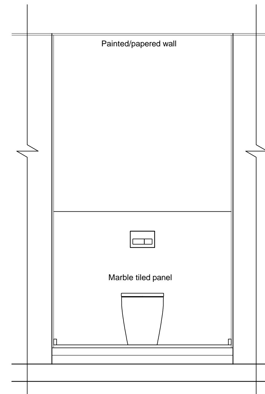
Elevation C
