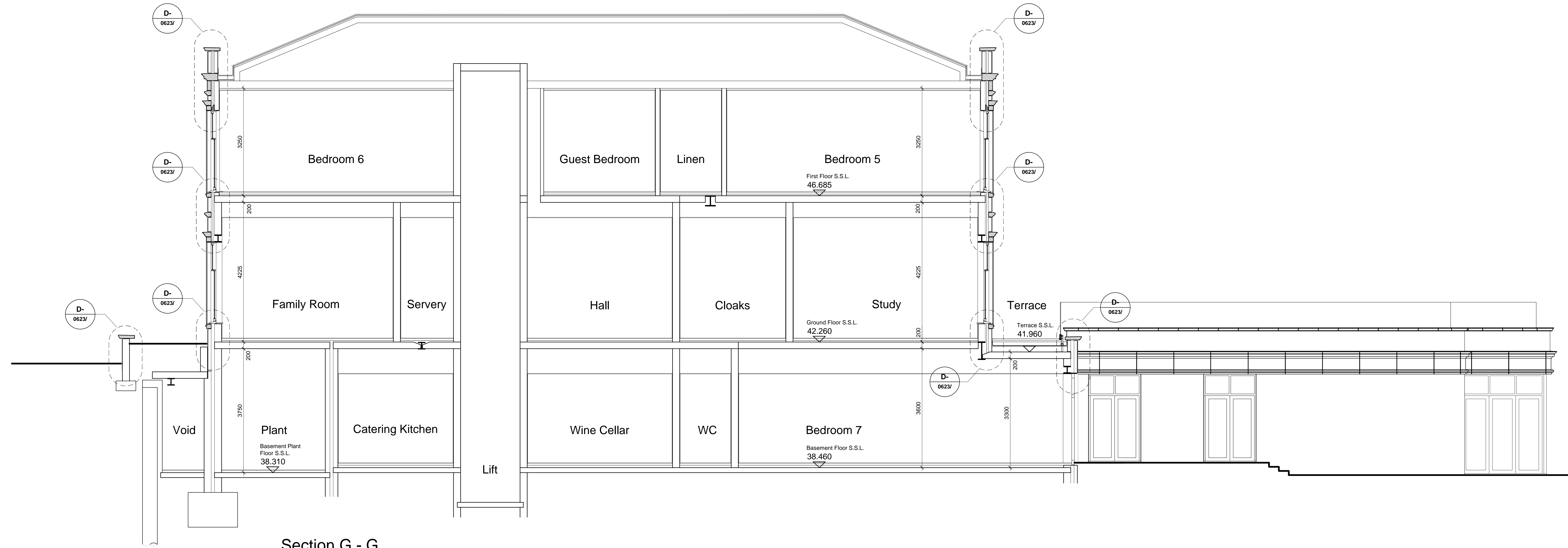
Section G - G
