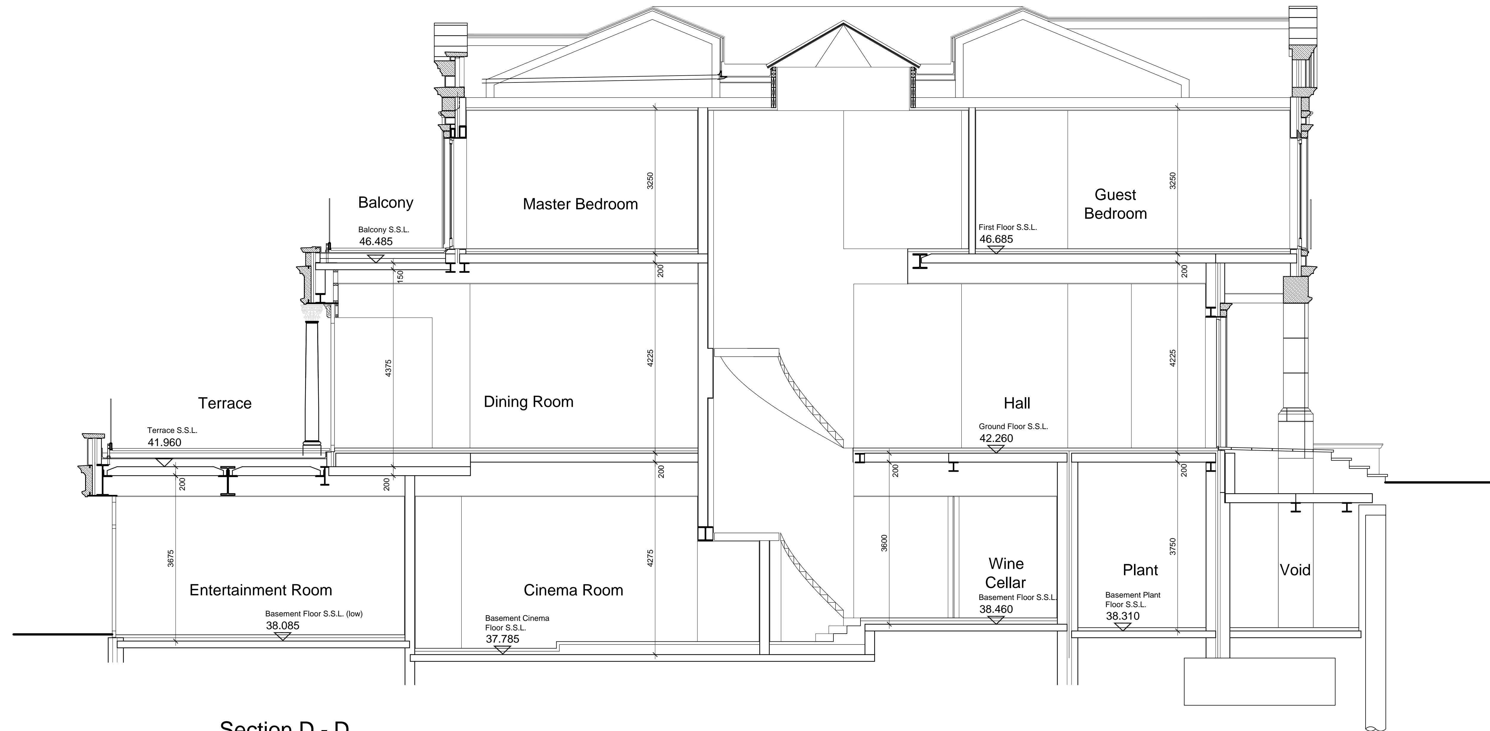
Section D - D
