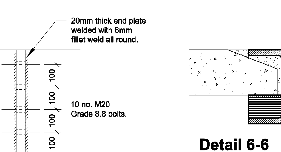
Detail 6-6
