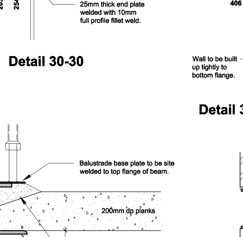
Detail 30-30
