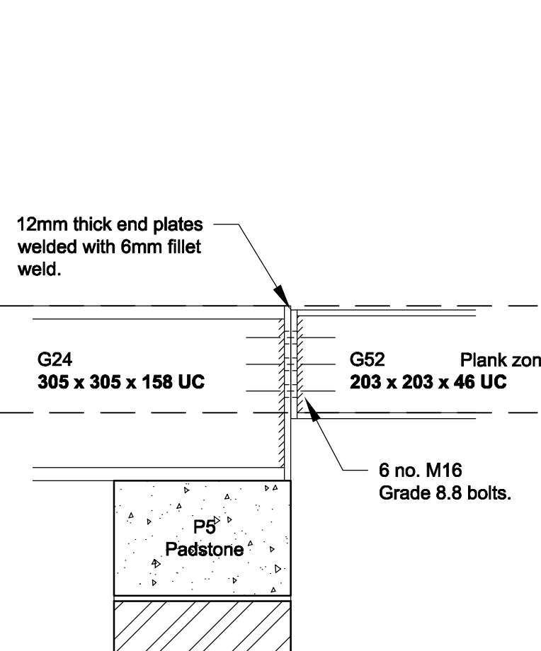
Detail 24-24
