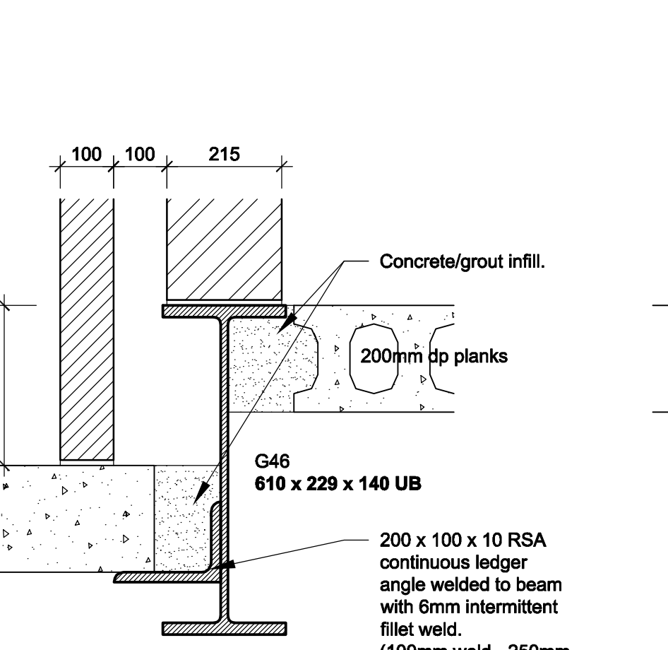
Detail 23-23
