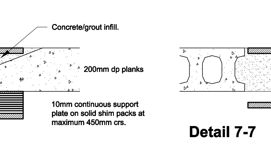
Detail 7-7
