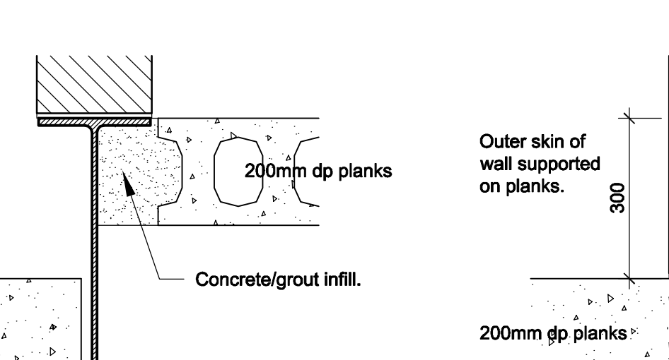
Detail 8a-8a
