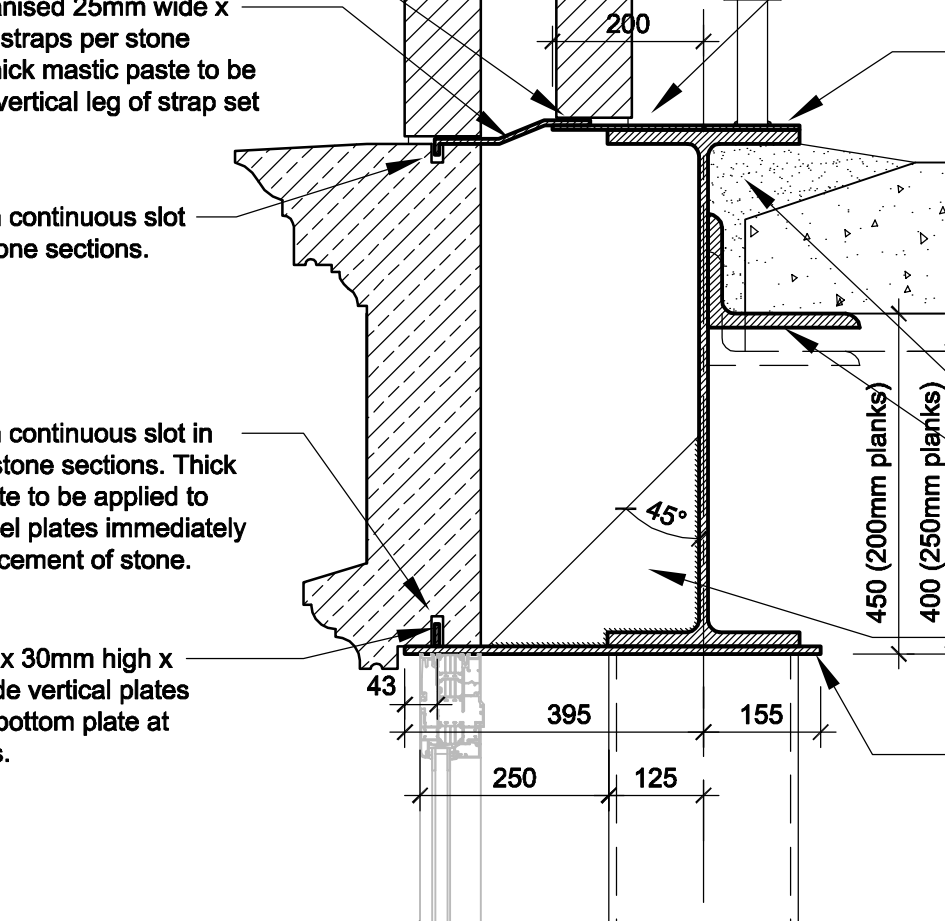
Detail 12-12
