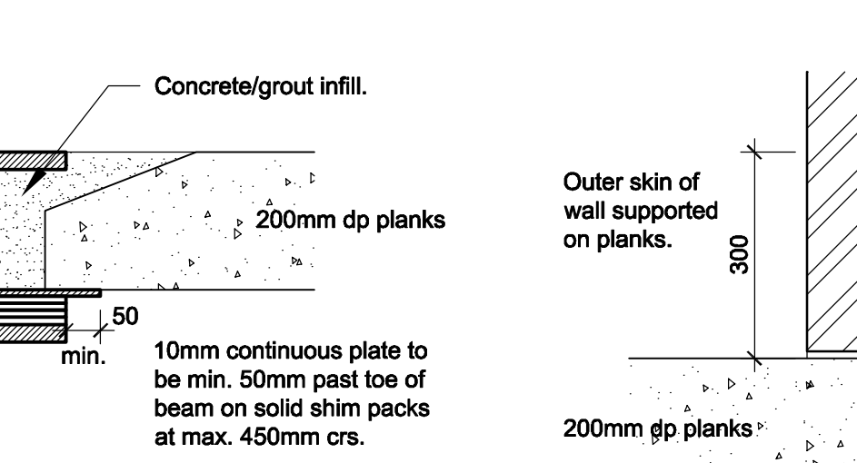
Detail 8-8
